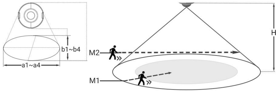
Installation diagram of CSBP-04/00.1.0x and CSBP-04/00.2.0
